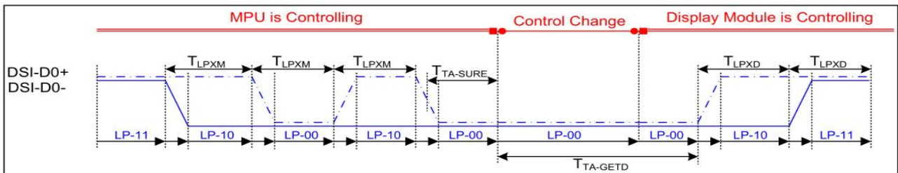
Figure 6 Bus Turnaround (BTA) from display module to MPU Timing
