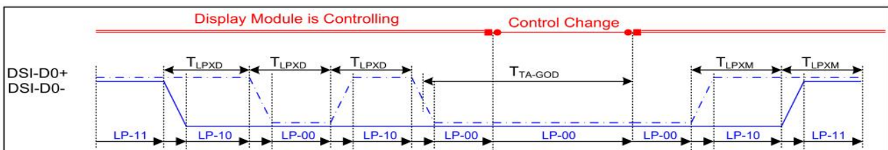
Figure 7 Bus Turnaround (BTA) from MPU to display module Timing
